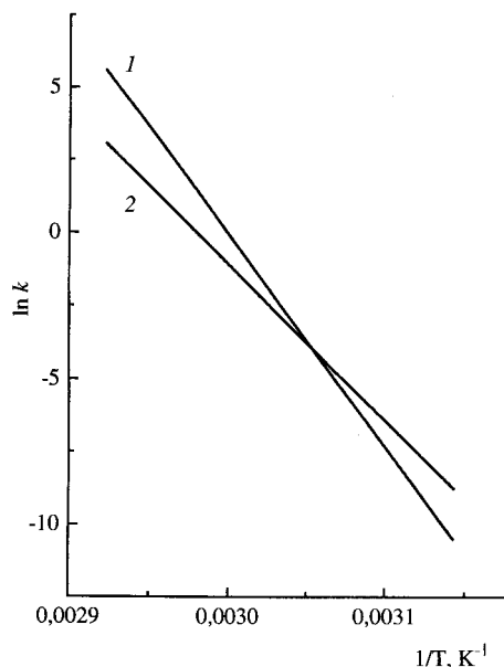
Fig. 2. Dependence of the rate constants for the first and second denaturation steps on the reciprocal temperature in semi-logarithmic coordinates for model (6). The values of Arrhenius equation parameters ( E_{a,1} = 609.3 kJ/mol, E_{a,2} = 446.8 kJ/mol, T_1^* = 333.4 K, T_2^* = 335.6 K) are taken from the results of simultaneous fitting to all the curves with the preliminary subtracted chemical baseline (see Table 3). The first and second step of the denaturation process are referred to as 1 and 2, respectively.
